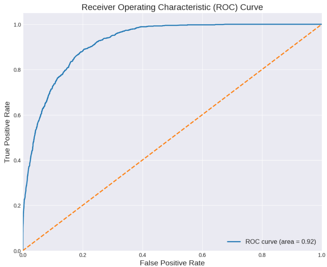
Gambar 4.27 Receiver Operating Characteristic (ROC) Curve
